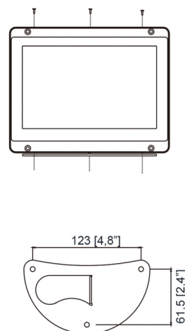
Hanging or Bracket mount (Bracket Optional)
